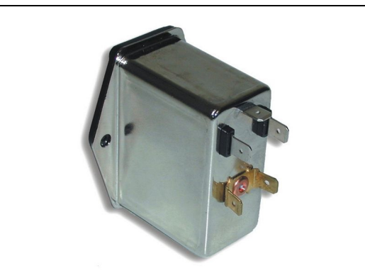
671.115.507 Linefilter 4A 3,15A incl. 2x fuse
